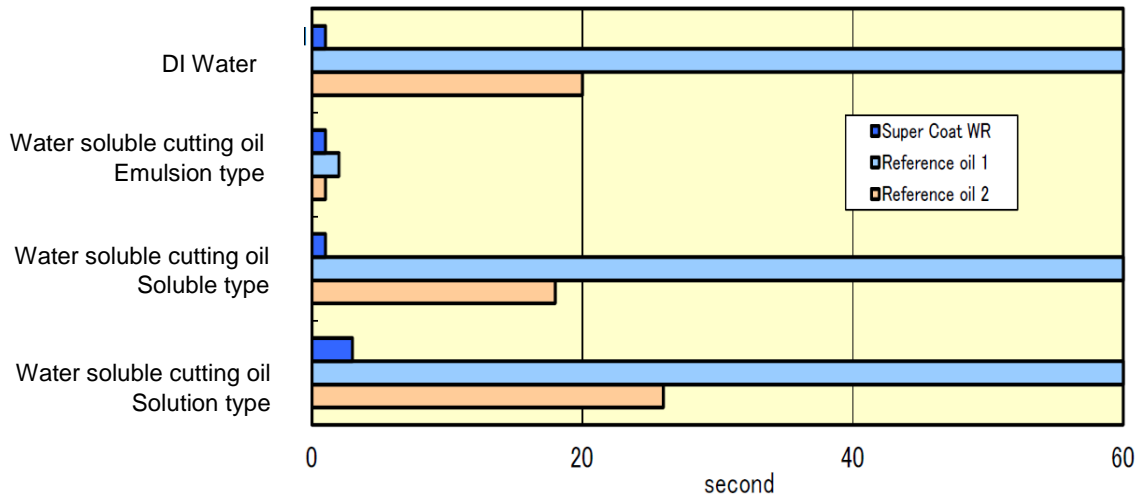
Figure: Water replacement test result between DAPHNE SUPER COAT WR and commercial in market test with DI water, Emulsion type water soluble cutting oil, Soluble type water soluble cutting oil, Solution type water soluble cutting oil
